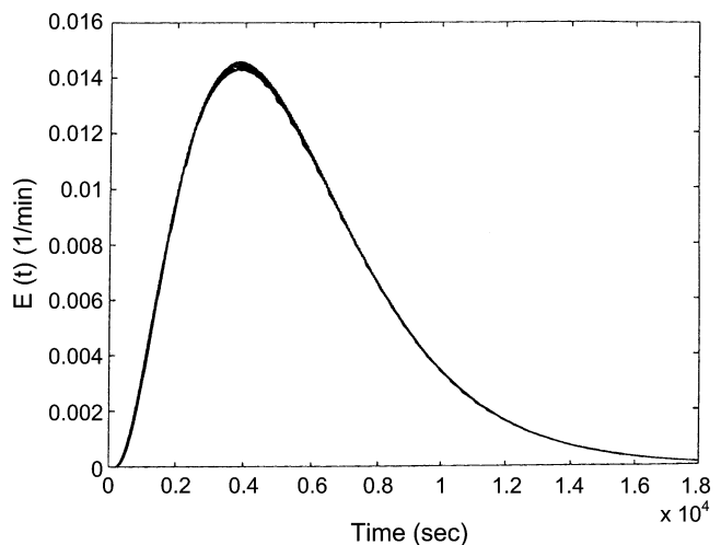
Fig. 9. Computed and experimental residence time distribution in the heavy phase of the bottom-gas-injected countercurrent liquid-liquid process [ \alpha=0.025 . Detailed test conditions are given in Iyer and Sohn, 1994].
